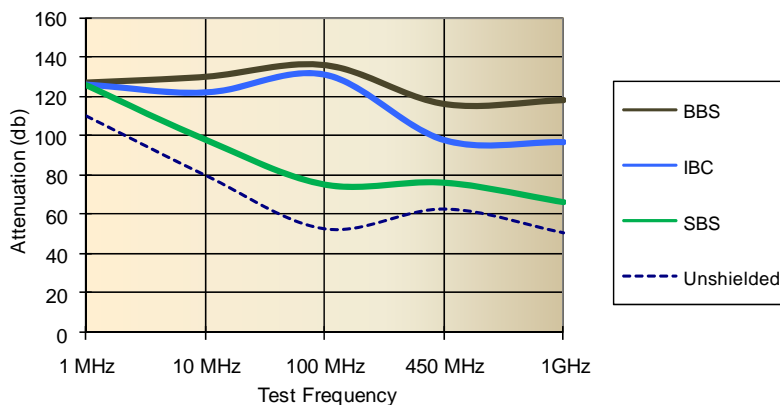
dBzSHIELD® Shielding Effectiveness
